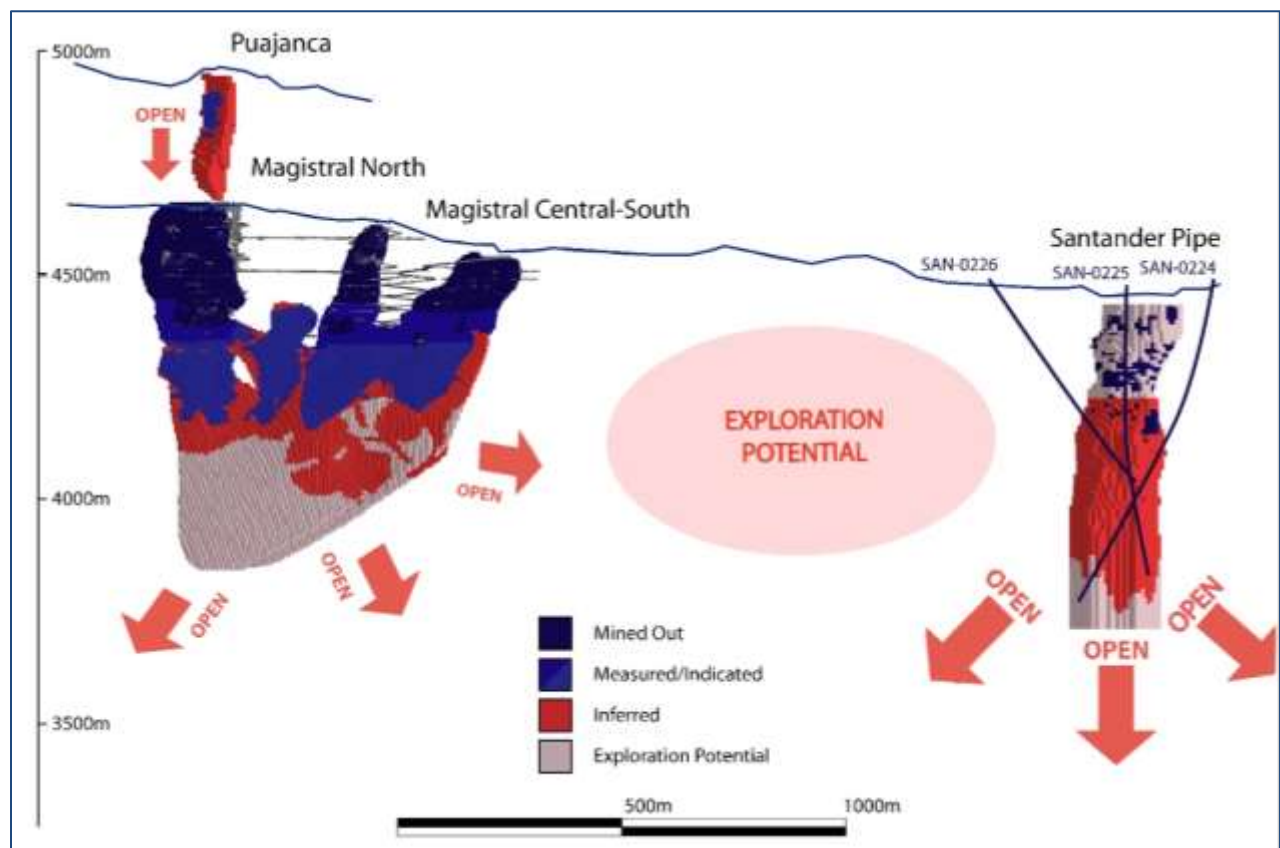
Figure 2: Longitudinal Section (Looking East) of Magistral Deposits, Puajanca and Santander Pipe targets
