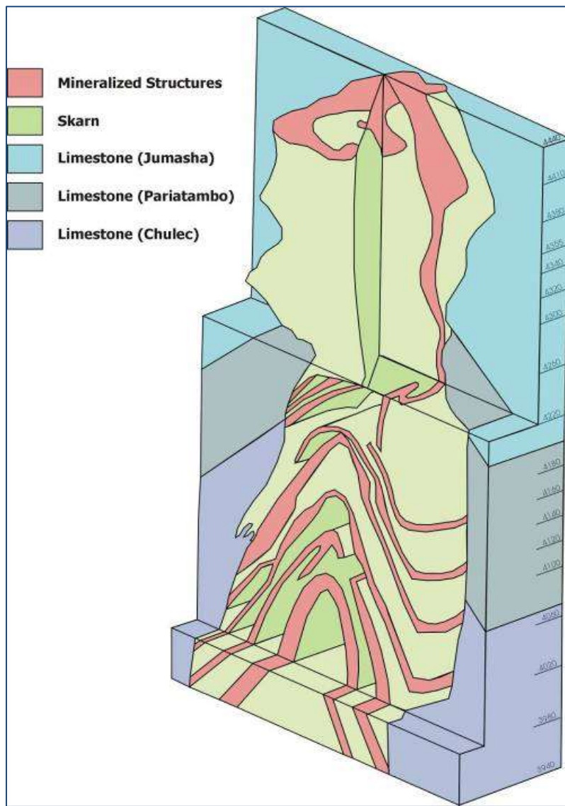
Figure 3: Schematic diagram of mineralization in former Santander Pipe mining operation.
