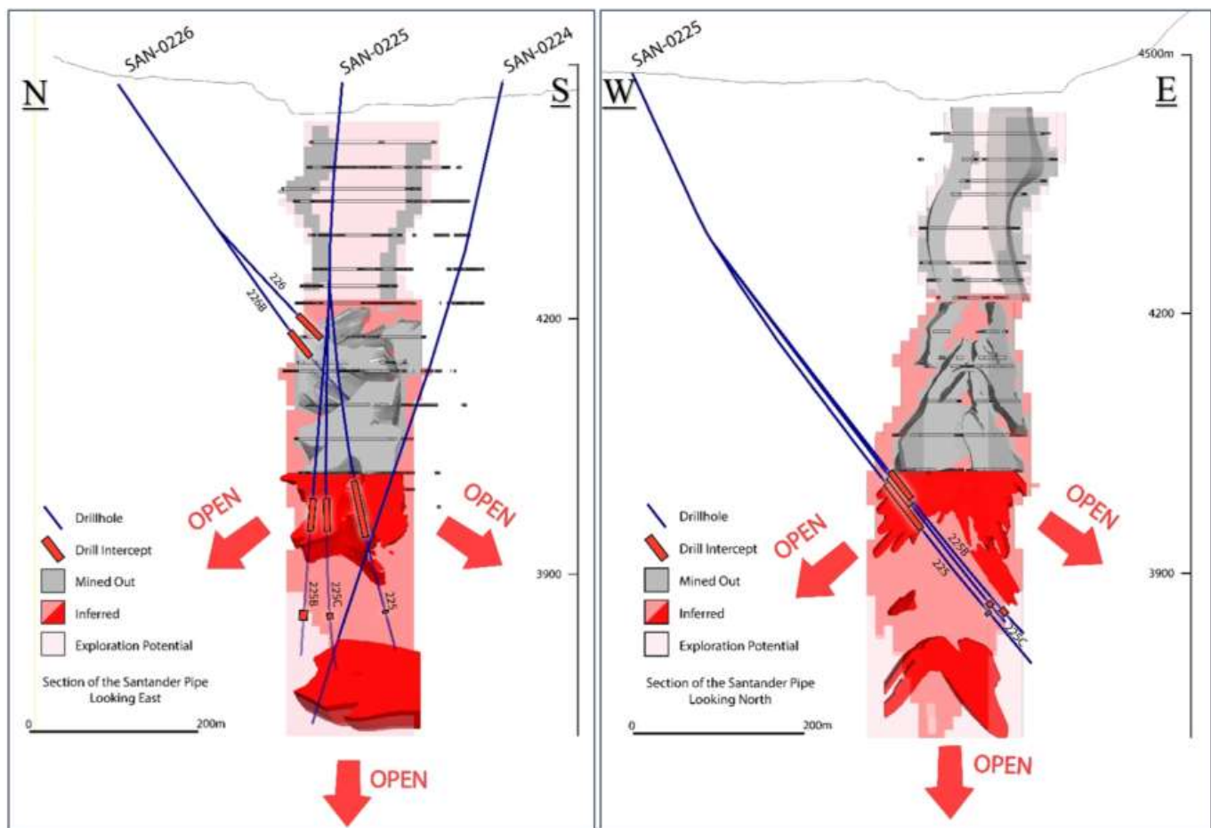
Figure 4 – Sections (N-S and W-E) through the Santander Pipe highlighting significant intersections as discussed in the text.
