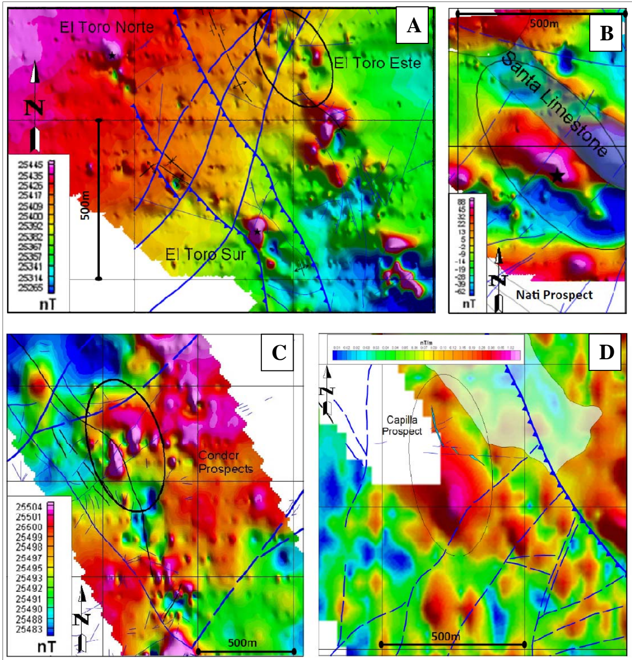
Figure 2: Detailed geophysical targets. A – Los Toros Prospects, B – Nati Prospect, C – Condor Prospect, D – Capilla Prospect. Maps A and C display total magnetic field. Map B displays total magnetic intensity and Map D displays (magnetic) analytical signal results
