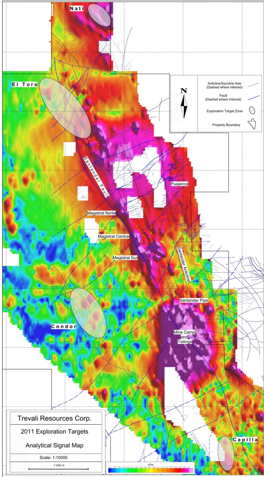
Figure 1: Magnetic (Analytical Signal) and summary Structural map of Santander Property showing location of priority targets.
