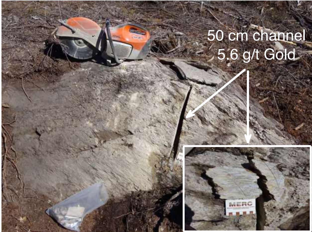
Figure 3. Conglomerate pebble bed in the new claims with assay of 5.6 g/t gold.
