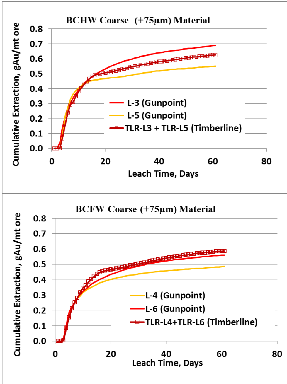
Figure 1. Interim Gold Leach Rate Profiles, Column Leach Tests of Agglomerated BCFW and BCHW Coarse (+75 \mu m) Material
