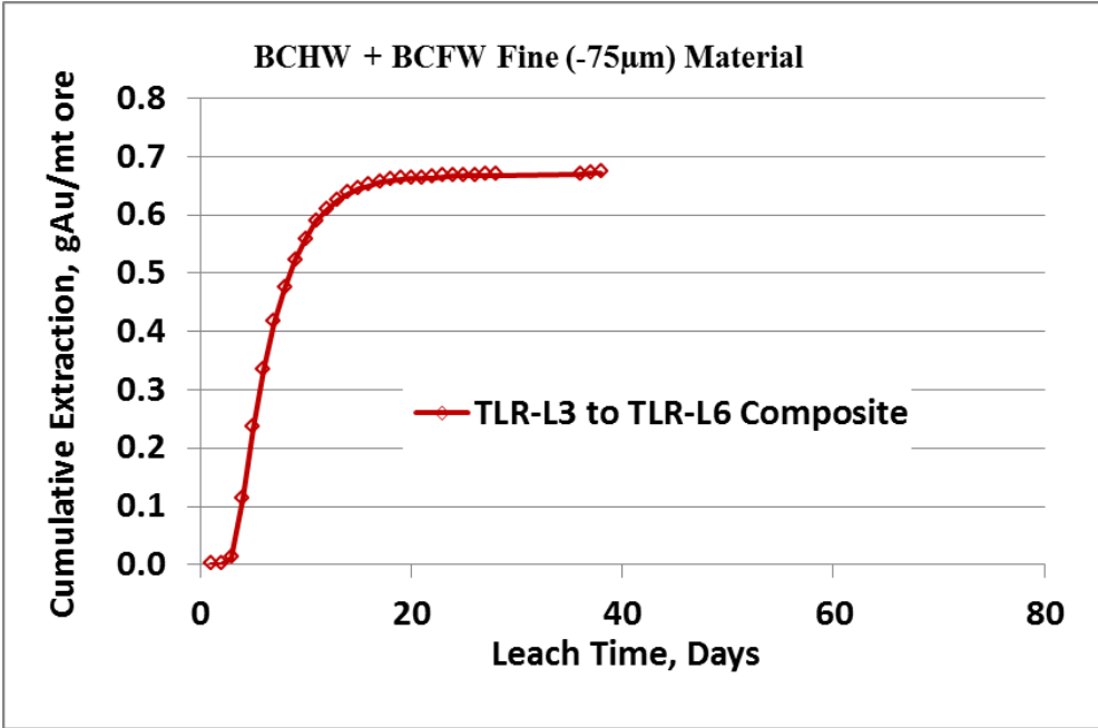
Figure 2. Interim Gold Leach Rate Profiles, Column Leach Tests of Agglomerated Composite of BCFW and BCHW Fine (-75µm) Material
