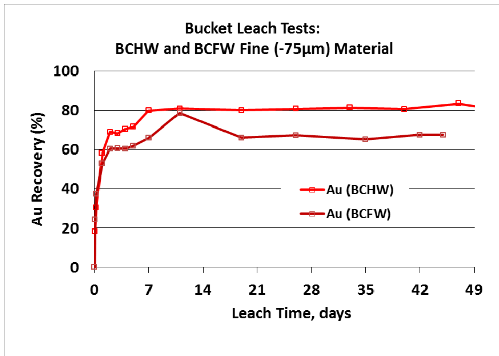
Figure 3. Interim Gold Leach Rate Profiles, Bucket Leach Tests of Agglomerated BCFW and BCHW Fine (-75 \mu m) Material
