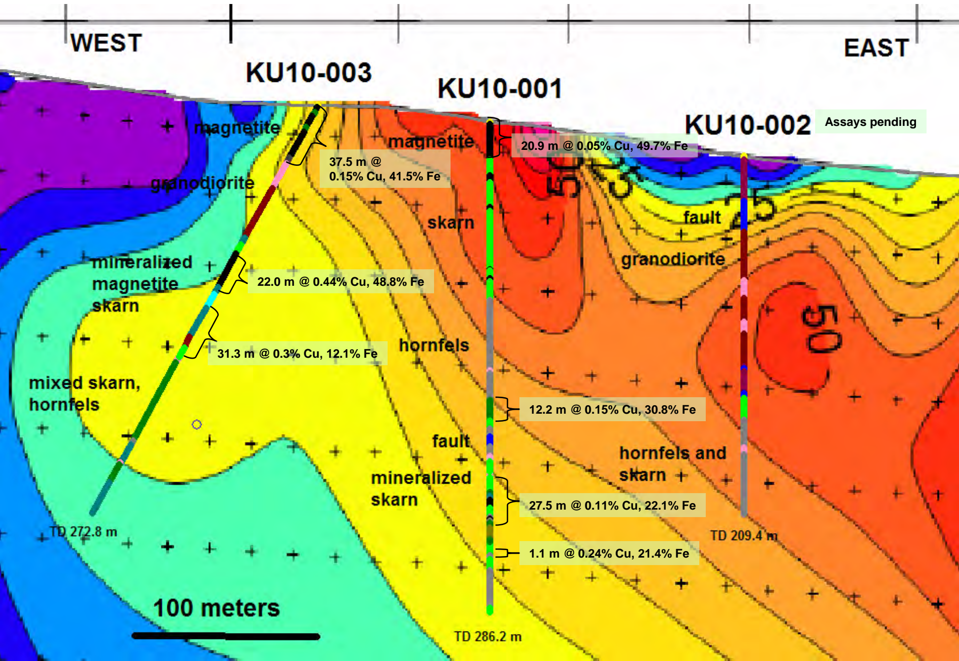
FIGURE 2 KUGRUK DRILLING AND IP GEOPHYSICS
