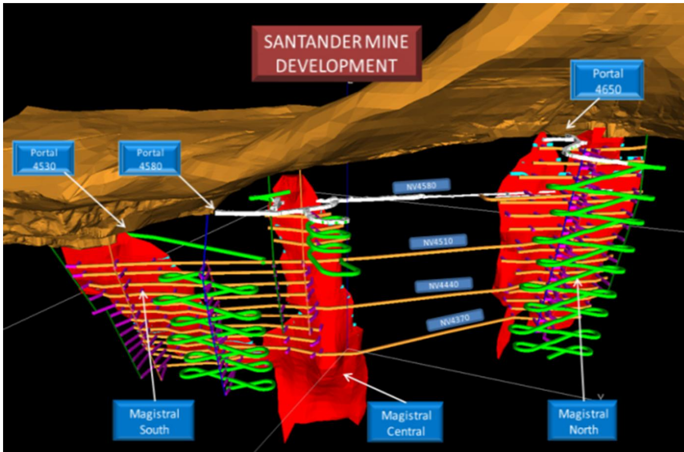
Figure 3: Santander Mine underground development plan (white portions of ramps completed to date)
