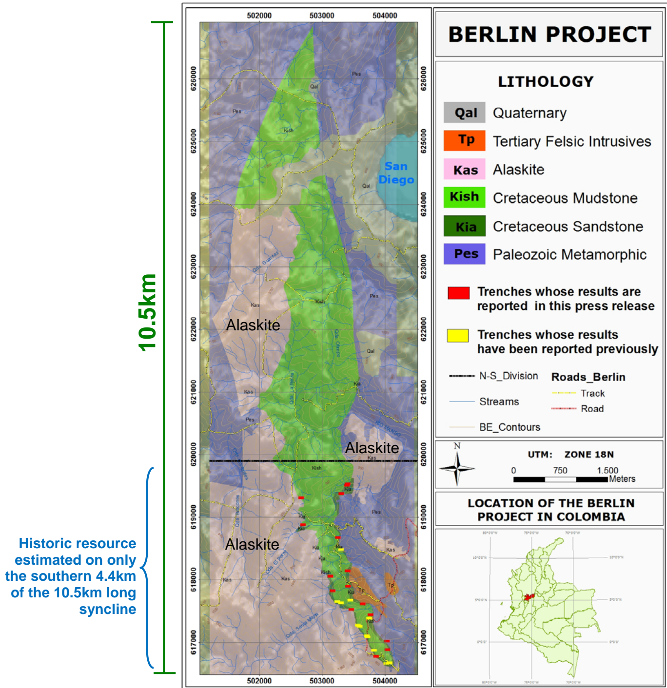
Geological map of the 10.5km long syncline of the Berlin Project in Caldas Province, Colombia. The pink coloured area shows the alaskite batholiths, the largest of which is located on the western flank of the syncline at Berlin.
