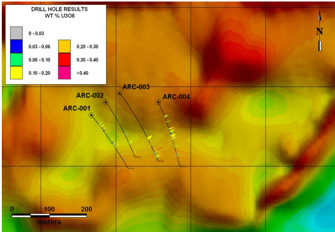
Figure 2 – Drill Hole Locations at Aricheng C
