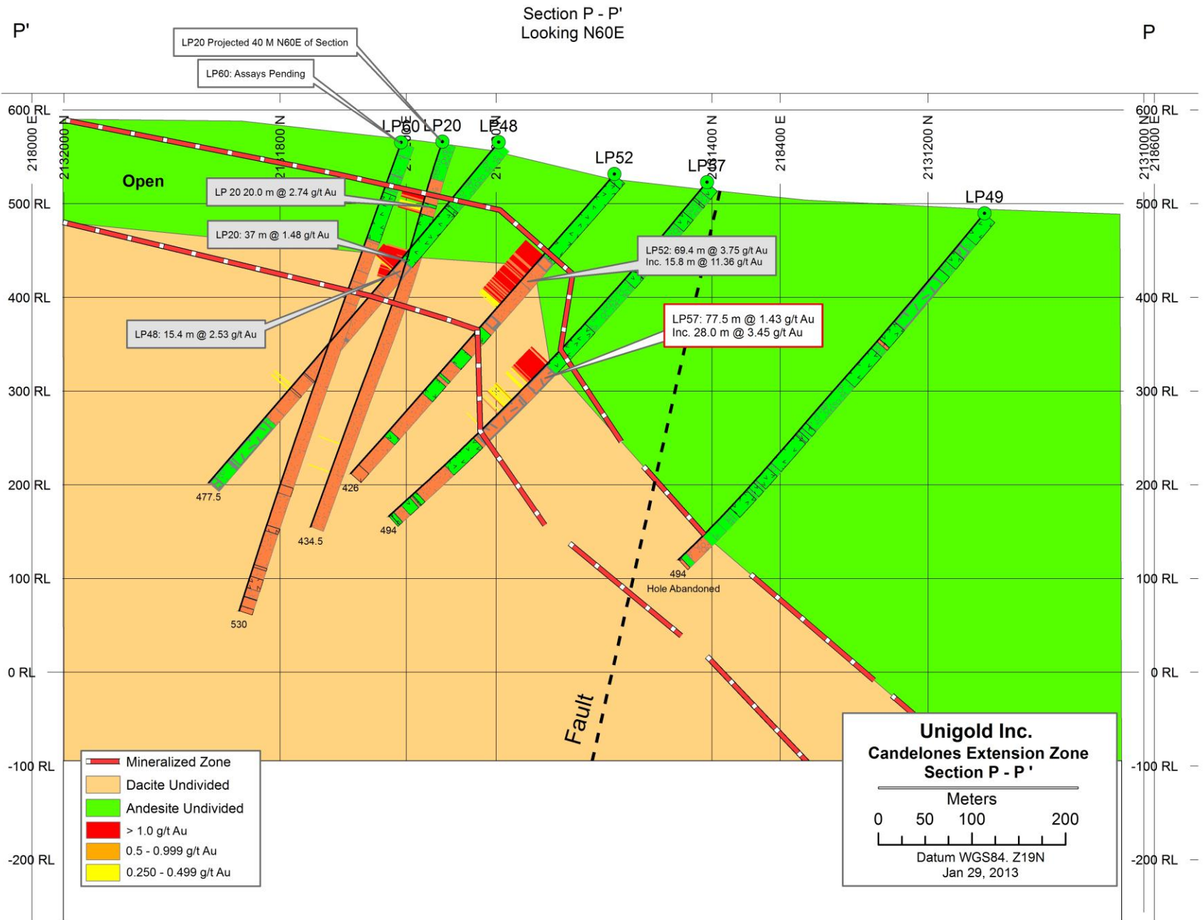
Figure 2: Section P-P'
