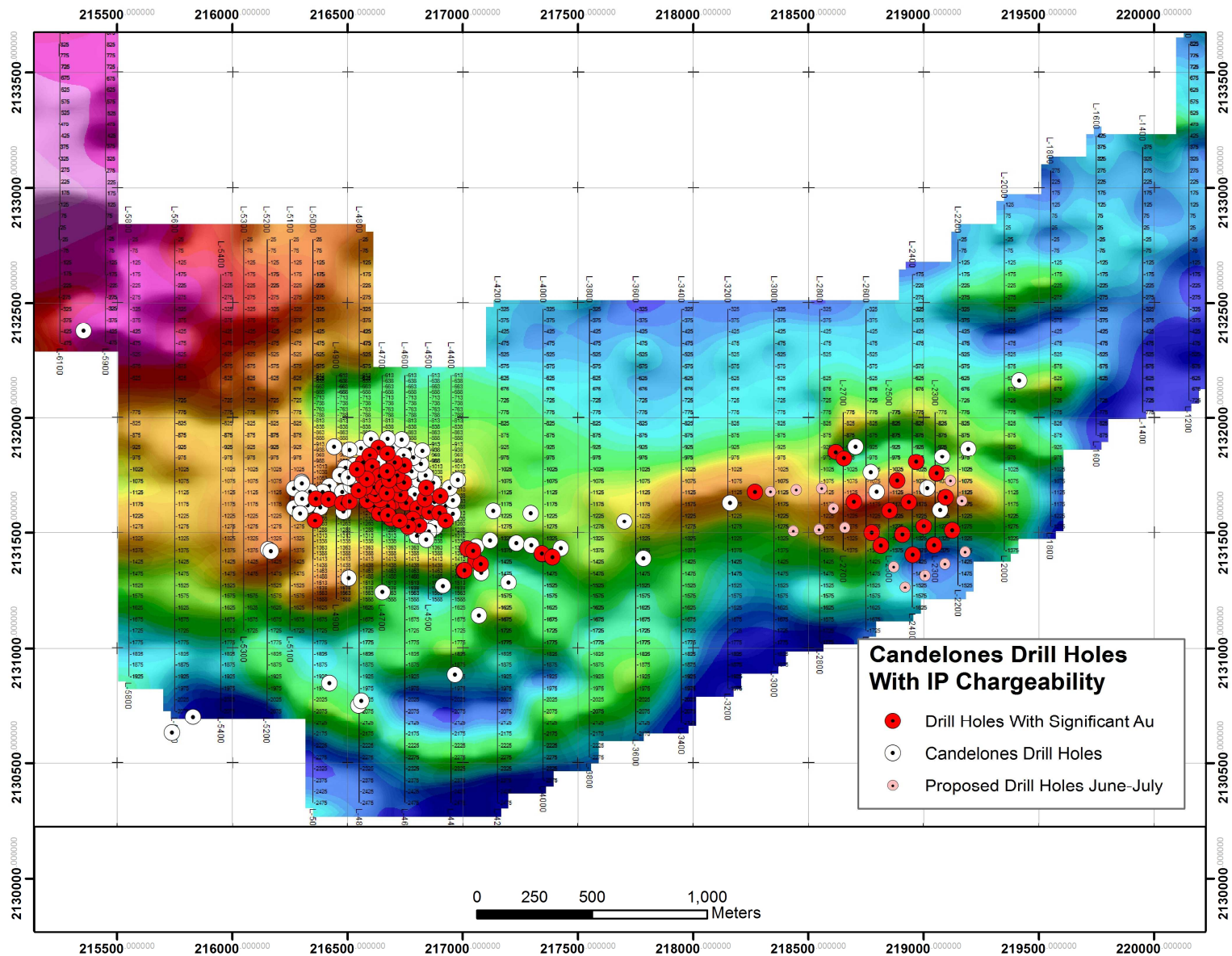
Figure 2: Candelones Drill Holes with IP Chargeability, Neita Concession, Dominican Republic
