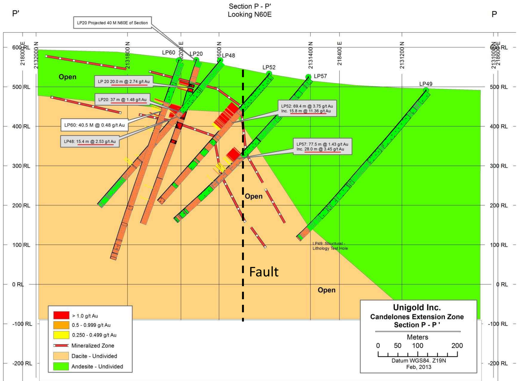
Figure 3: Section P-P'
