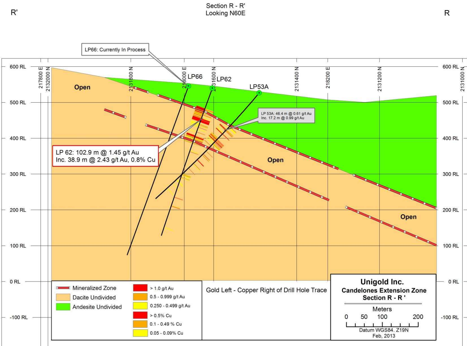
Figure 2: Section R-R'
