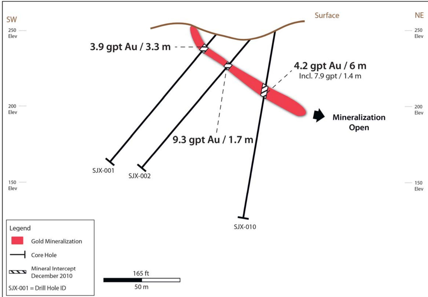
Figure 3 San Jose del Alamo Cross Section – Section Number: NESW North 20
