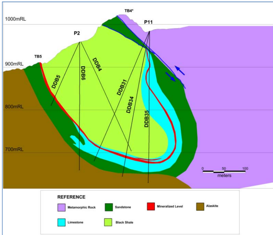
Figure 3 – Cross Section 3
