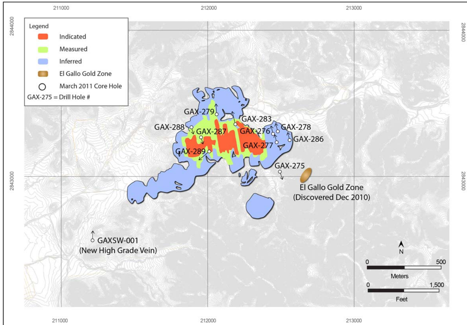
Figure 2 El Gallo Mineralization: Plan (Aerial View)
