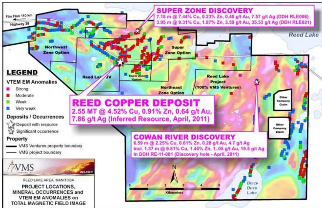
Figure 1 – Project Locations, Mineral Occurrences and VTEM EM Anomalies on Total Magnetic Field Image
