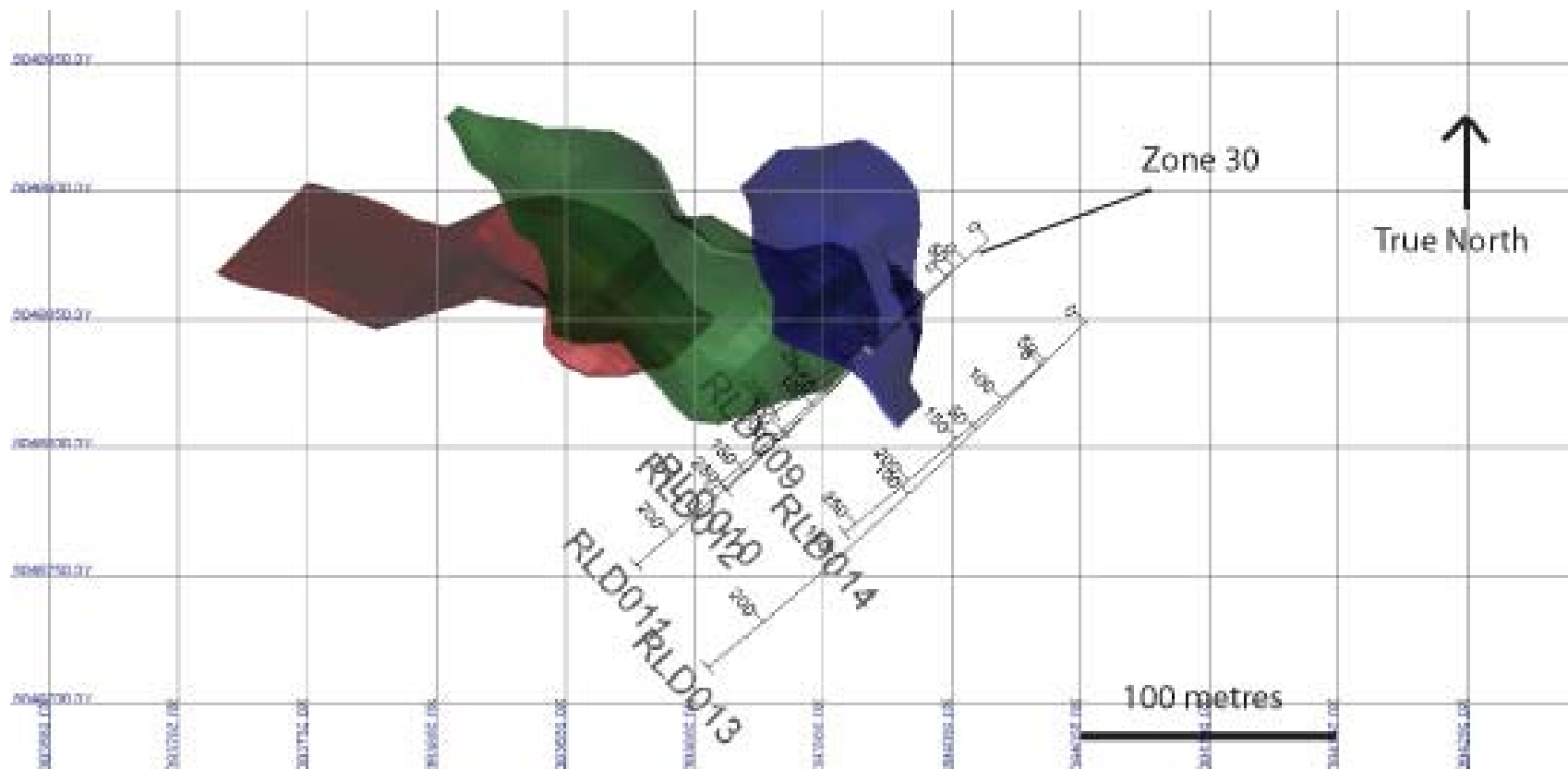
Figure 1, plan view of mineralized zones and drill holes RLD009 to RLD014 inclusive.
