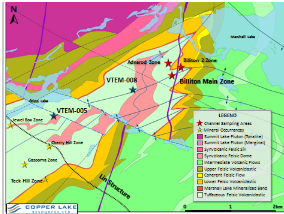
Figure 1: Marshall Lake: Prospect Location Map
