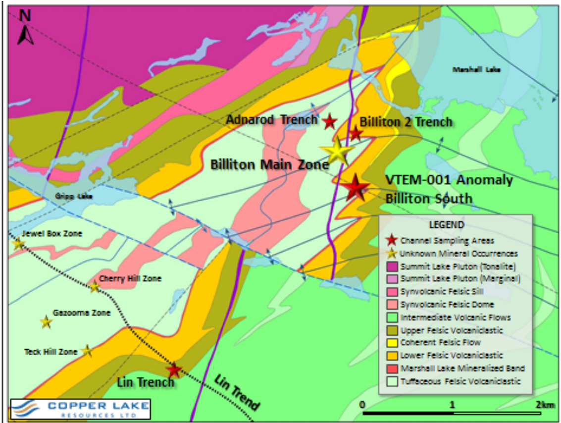
Figure 2: Billiton Main Zone Location
