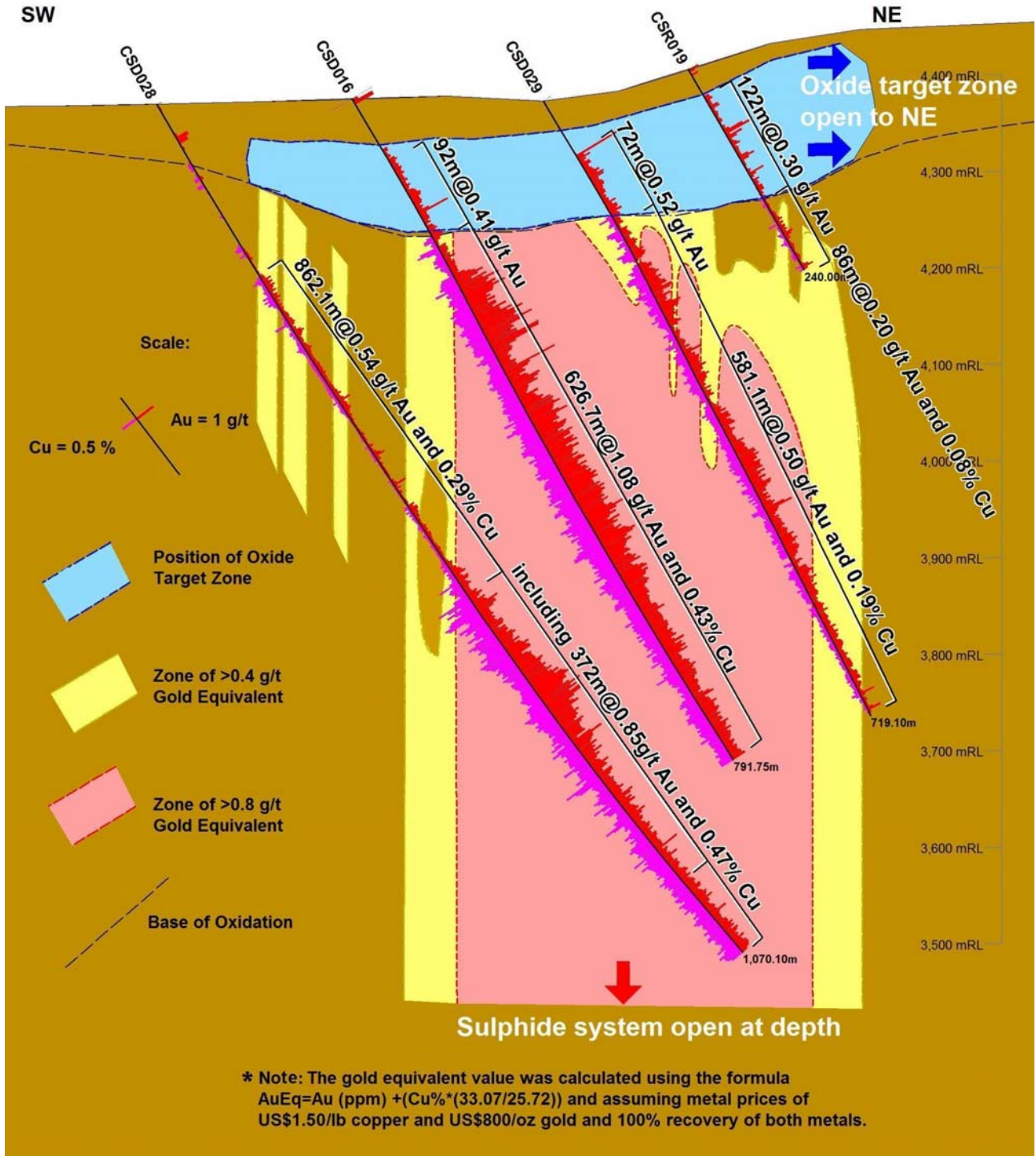
Figure 2 Drill section showing results and interpreted gold equivalent grade contours for holes CSD028, CSD016, CSD029 and CSR019.
