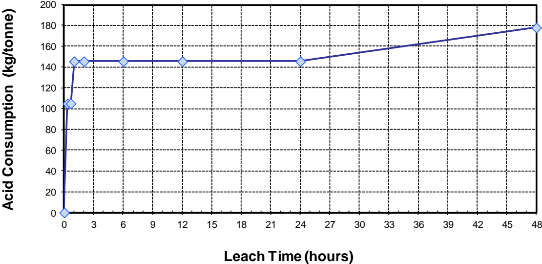
Figure I: Bottle roll test results for Pinocho-1 (in 100 g/l acid solution)
