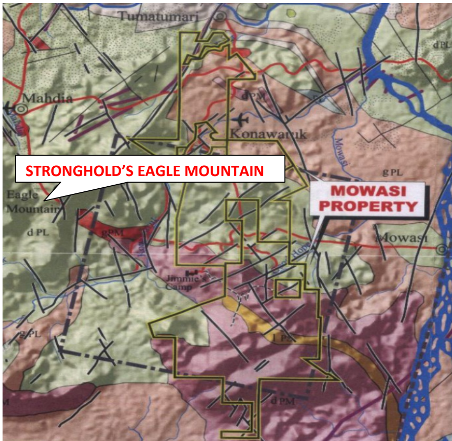
Figure 1: Regional Geology of the Mowasi and Eagle Mountain areas (from Alexander, 2011)
