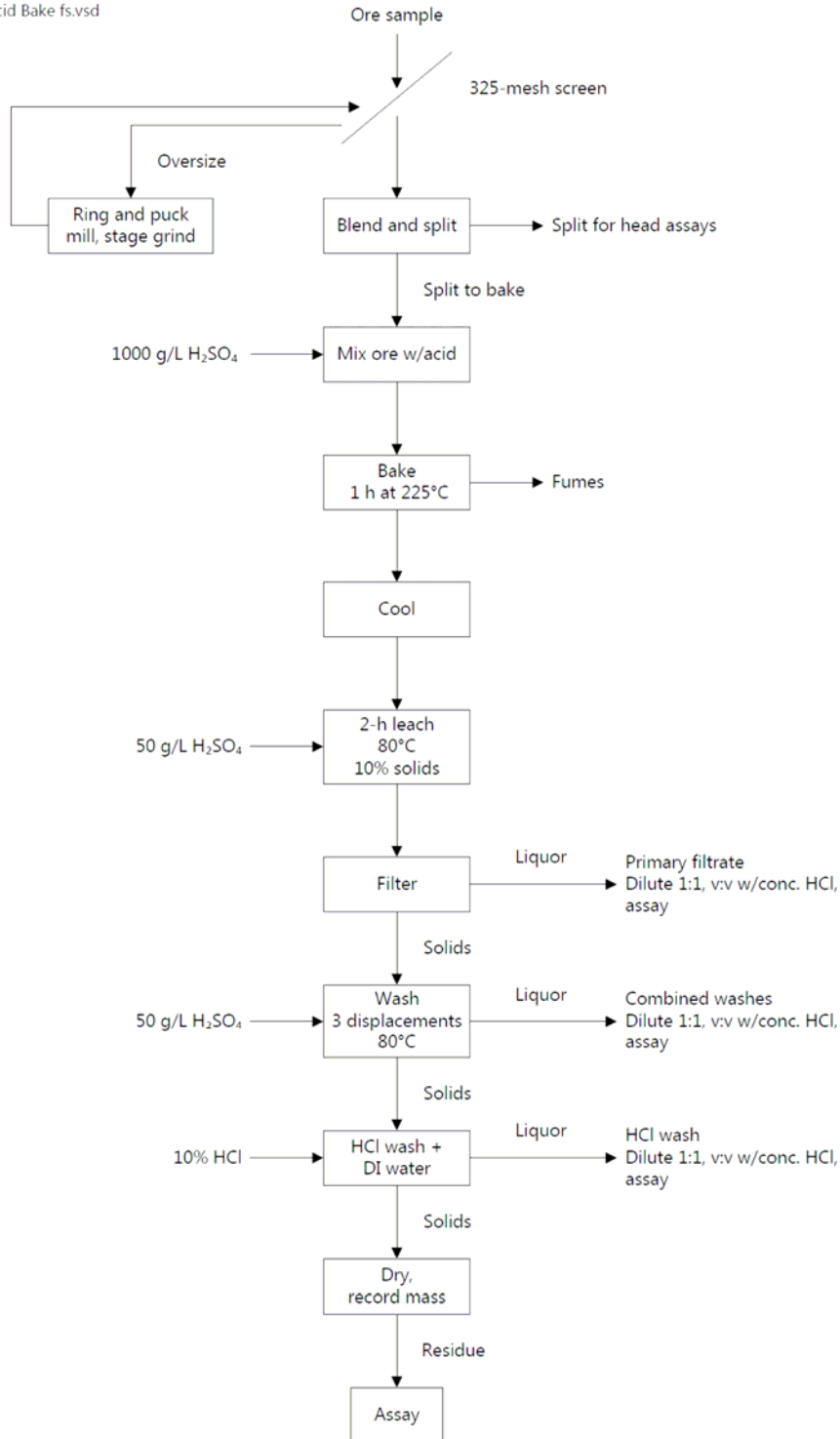
Flowsheet for Acid Bake and Leach Experiment
