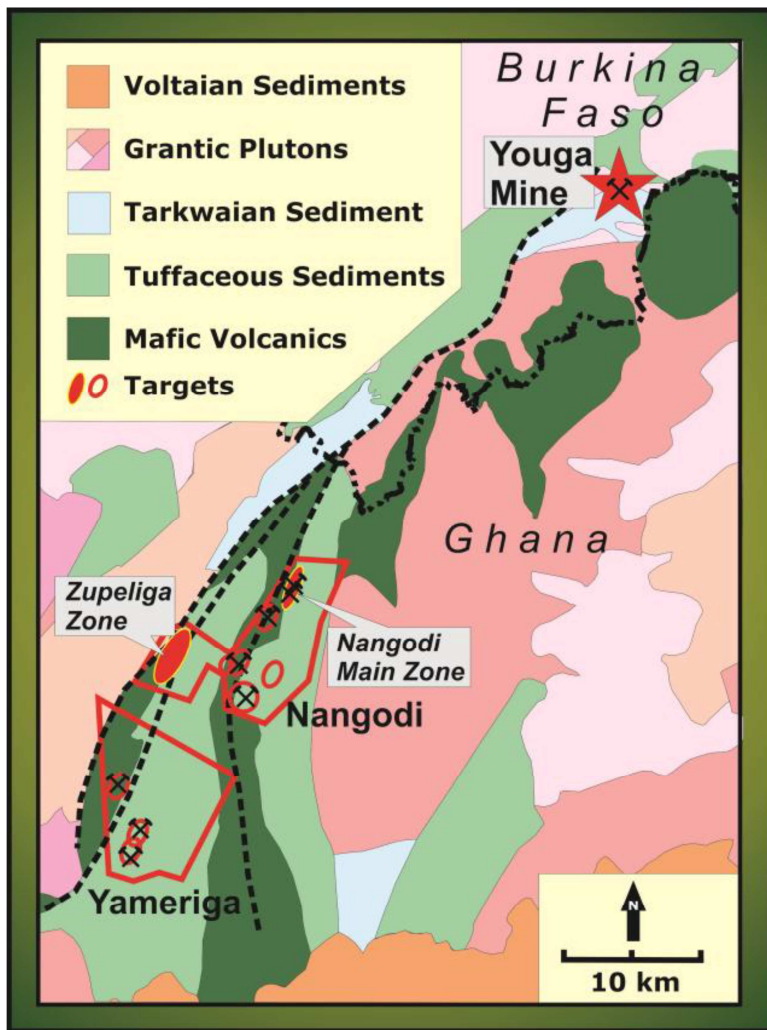
Figure 1. Regional geologic map showing the Nangodi and Yameriga concessions. Nangodi Main Zone and other satellite mineralized zones lie along the Nangodi Shear zone. Zupeliga lies along a parallel shear zone. (Source: Abzu Gold)
