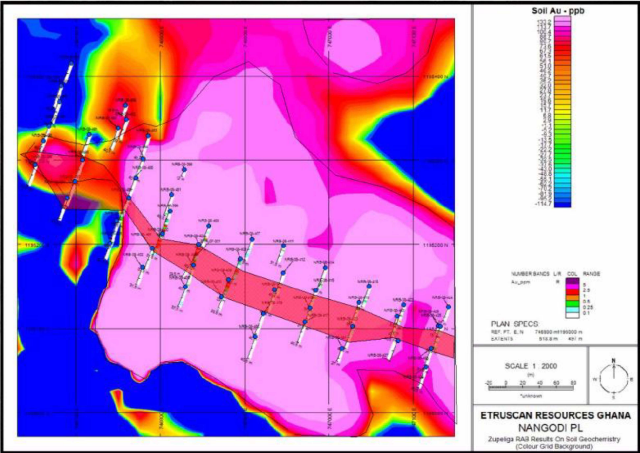
Figure 2. Zupeliga geochemical map showing gold in surface samples and the mineralized zone intersected in historic (2008) Etruscan RAB drill holes. (Source: Etruscan Resources, 2008)
