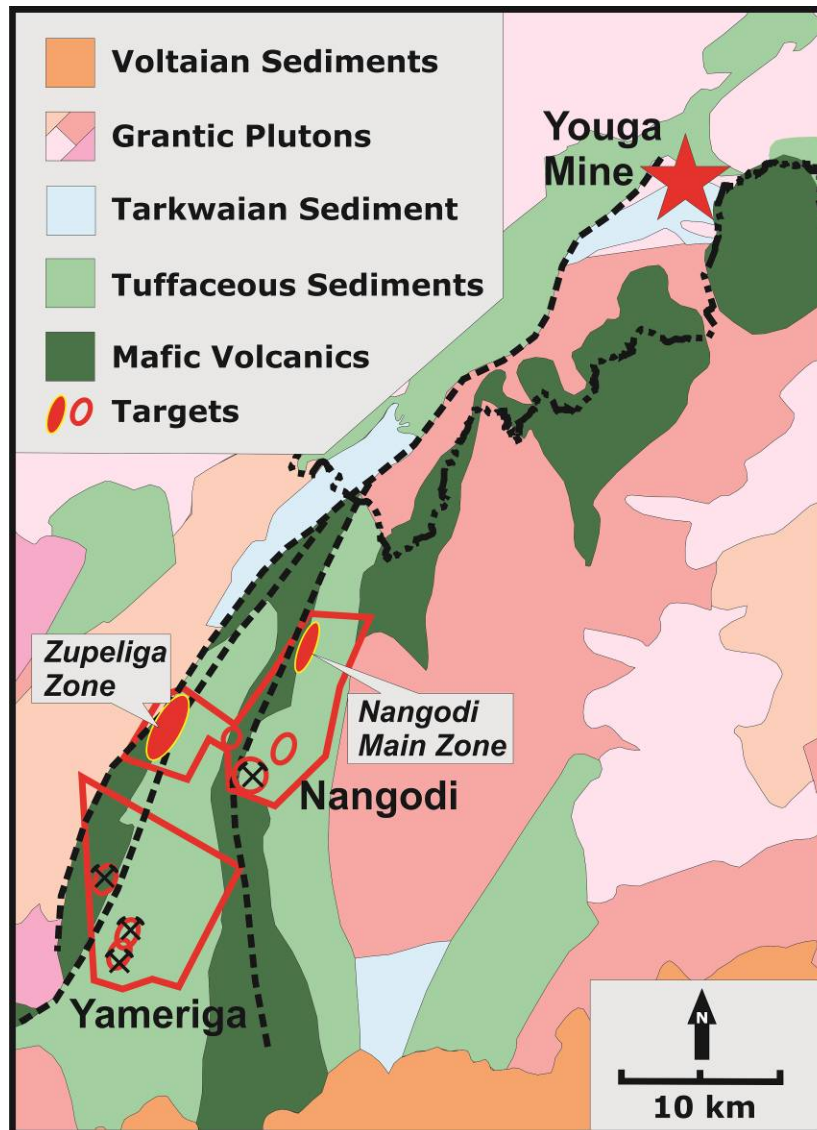
Figure 2. Location map showing Nangodi and Yameriga concessions. The Youga Mine in Burkina Faso lies along strike within the belt.
