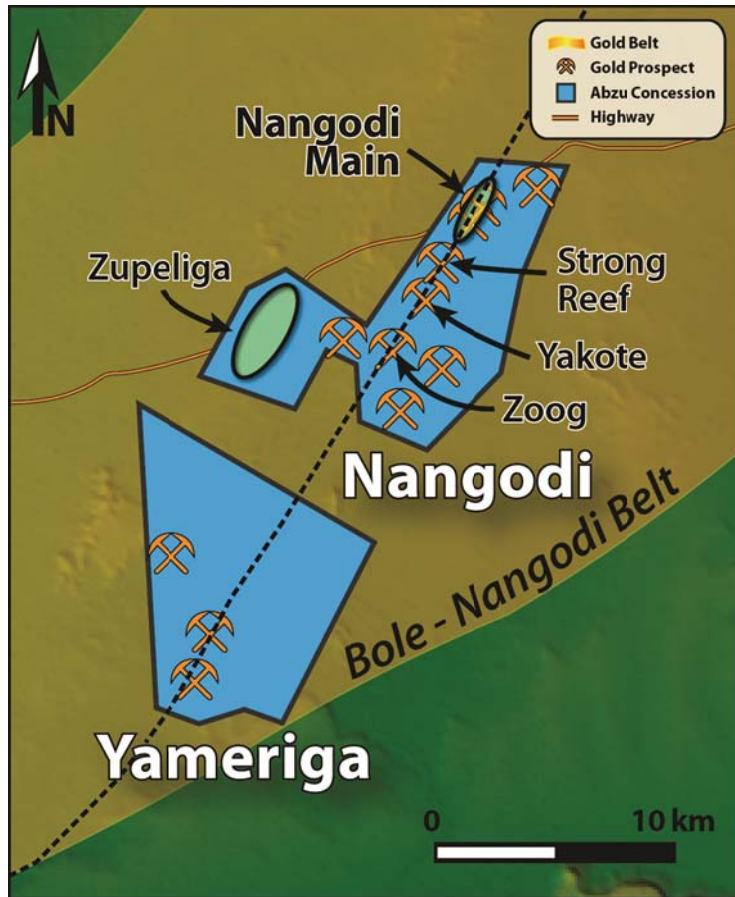
Figure 2: The Nangodi Main project area is one of numerous targets within the Nangodi and Yameriga concessions. The Youga Mine in Burkina Faso is on the same shear zone (dashed line) as Nangodi Main and other targets.
