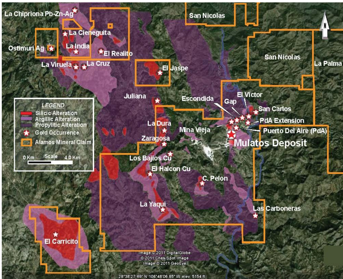
Figure 2: Mulatos District Property Alteration and Known Gold Occurrences
