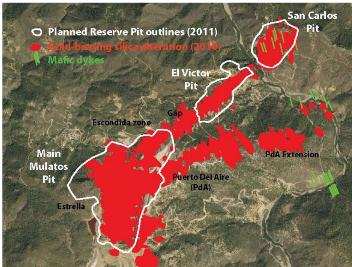
Figure 1: Mulatos Pit Area
