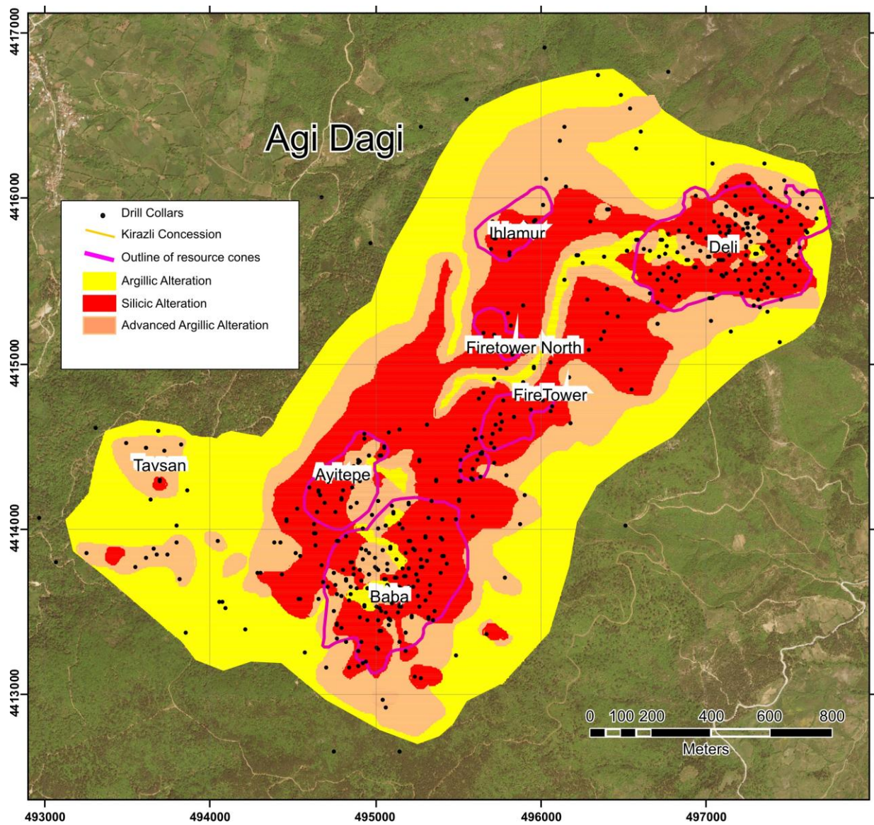
Figure 3: Ağı Dağı Project Alterations and Known Gold Occurrences
