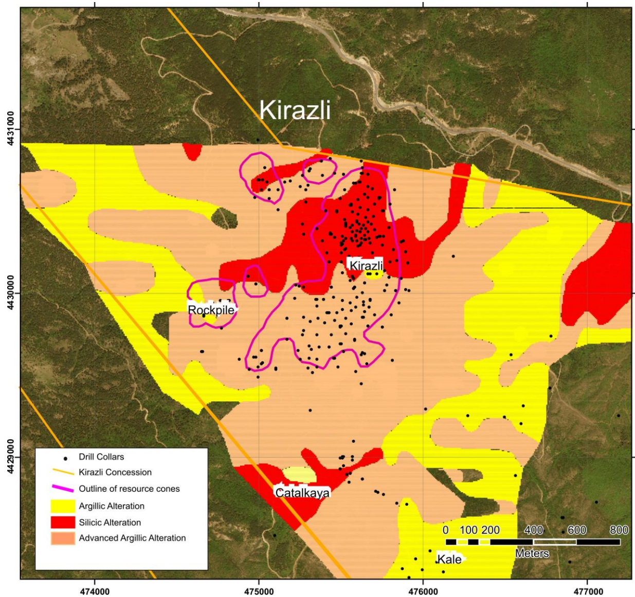
Figure 5: Kirazlı Project Alteration and Known Gold Occurrences
