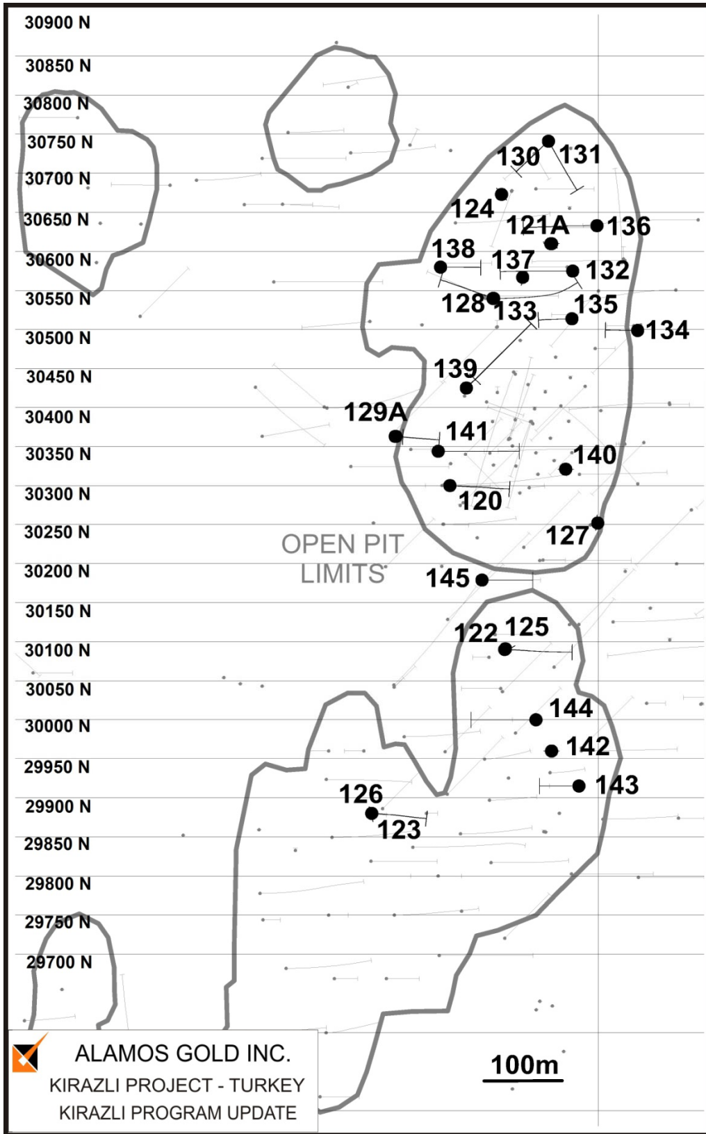
Figure 6: Kirazlı - Drill Hole Locations
