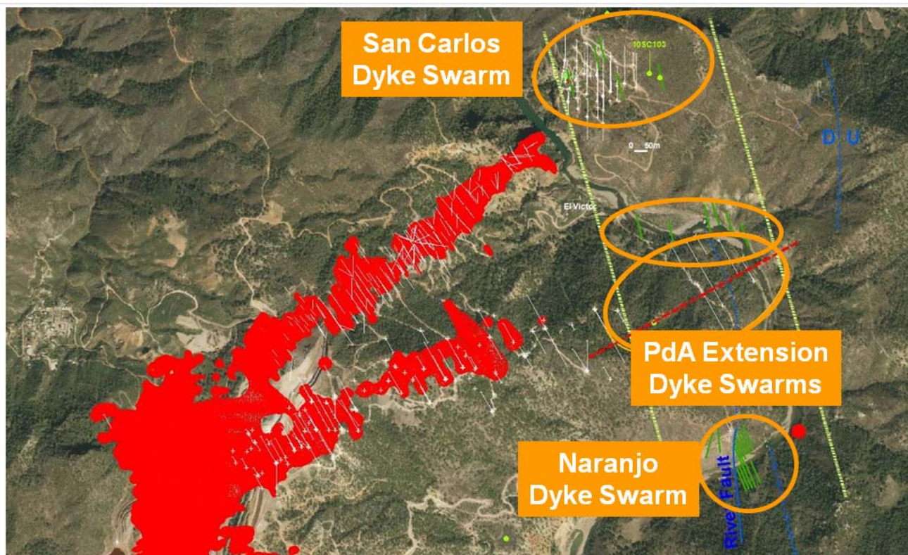
Figure 4: Near-Mine Mafic Dyke Swarm Locations
