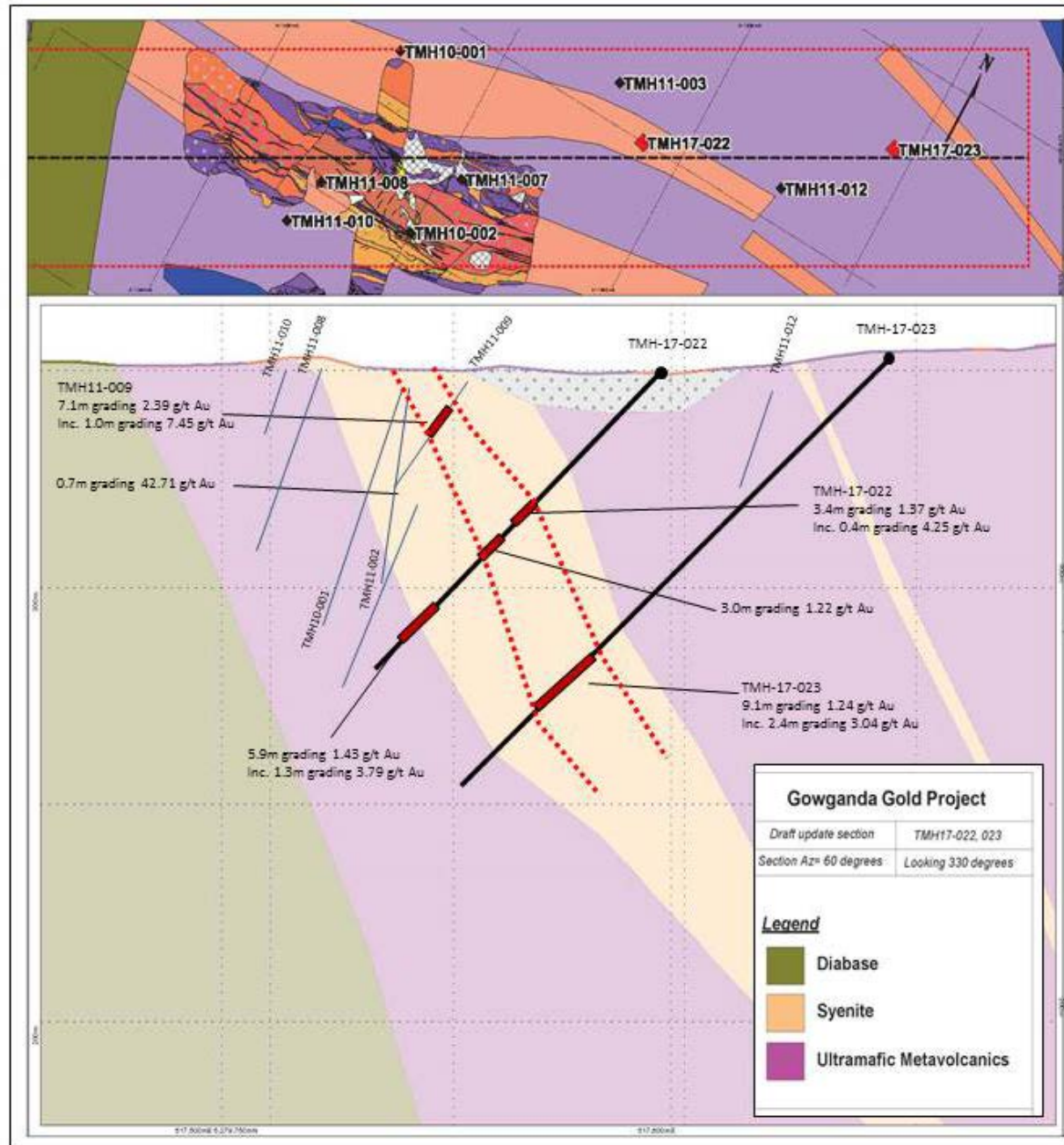
Figure 2. Section A-A' Looking Northwest
