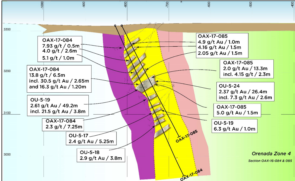
Figure 2. Cross Section, DDH OAX-17-084 and 085
