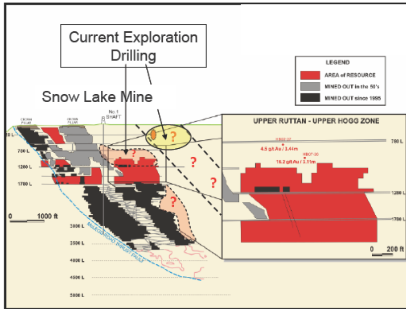
Figure 1: Longitudinal Section of the Snow Lake Mine, Manitoba (formerly the New Britannia Mine). Mine workings, areas of past production and current Resources projected to a vertical plane, viewed to north-northwest.
