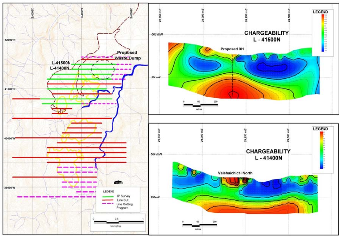
Figure 3 Gold Ridge Project Exploration – IP Survey – Chargeability response over northern end of Valehaichichi deposit and proposed VAL_OSF site (broken black line on plan)
