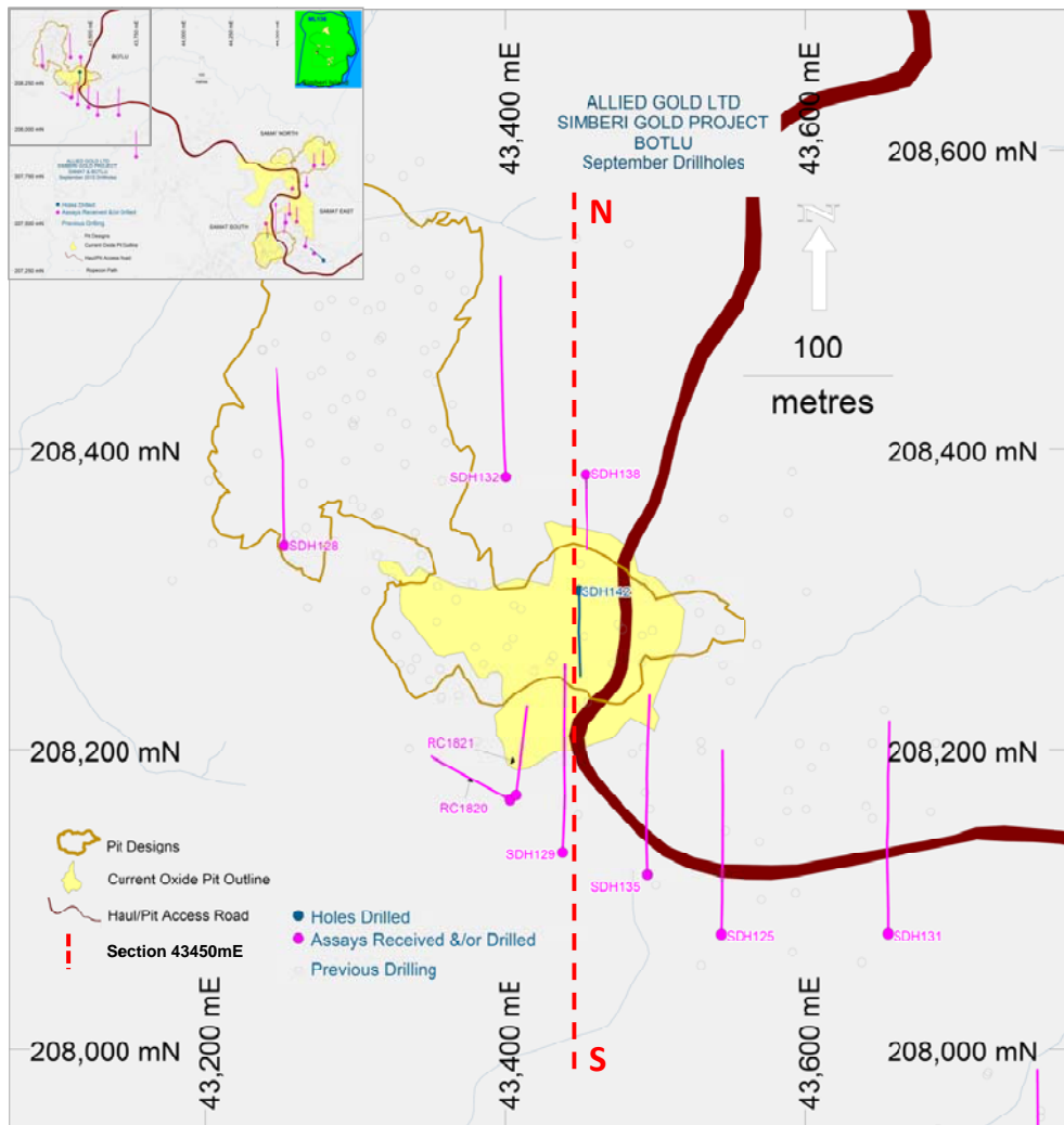
Figure 4 Botlu Prospect - Collar and traces of holes drilled prior to (grey) and during Sep 2010 Qtr(magenta drilled – assays received; blue = drilled / assays awaited)
