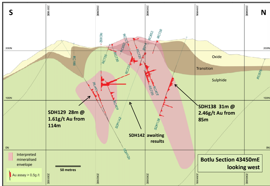
Figure 5 BotluDeposit – N-S section (looking west) illustrating gold intersections in core holes SDH129 and SDH138.
