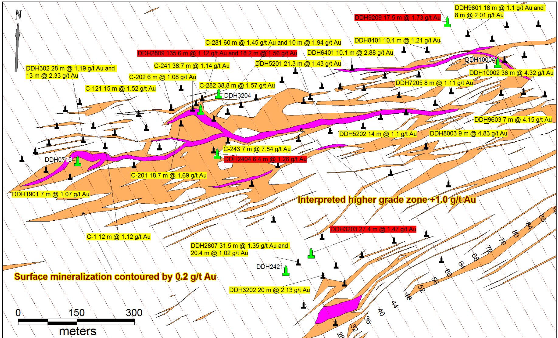
Figure 2 – Shirotnaia 2007-2012 Drilling Results (with intercepts of grades greater than or equal to 1.0 g/t Au and widths greater than or equal to 7.0 m) and Core Hole Positions (2012 reported holes – green towers)
