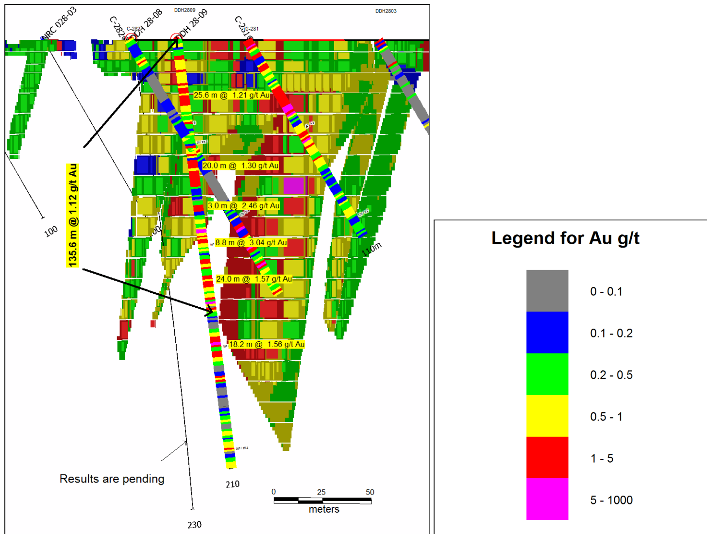
Figure 3 – NW-SE cross section through hole DDH 28-09 along line 28
