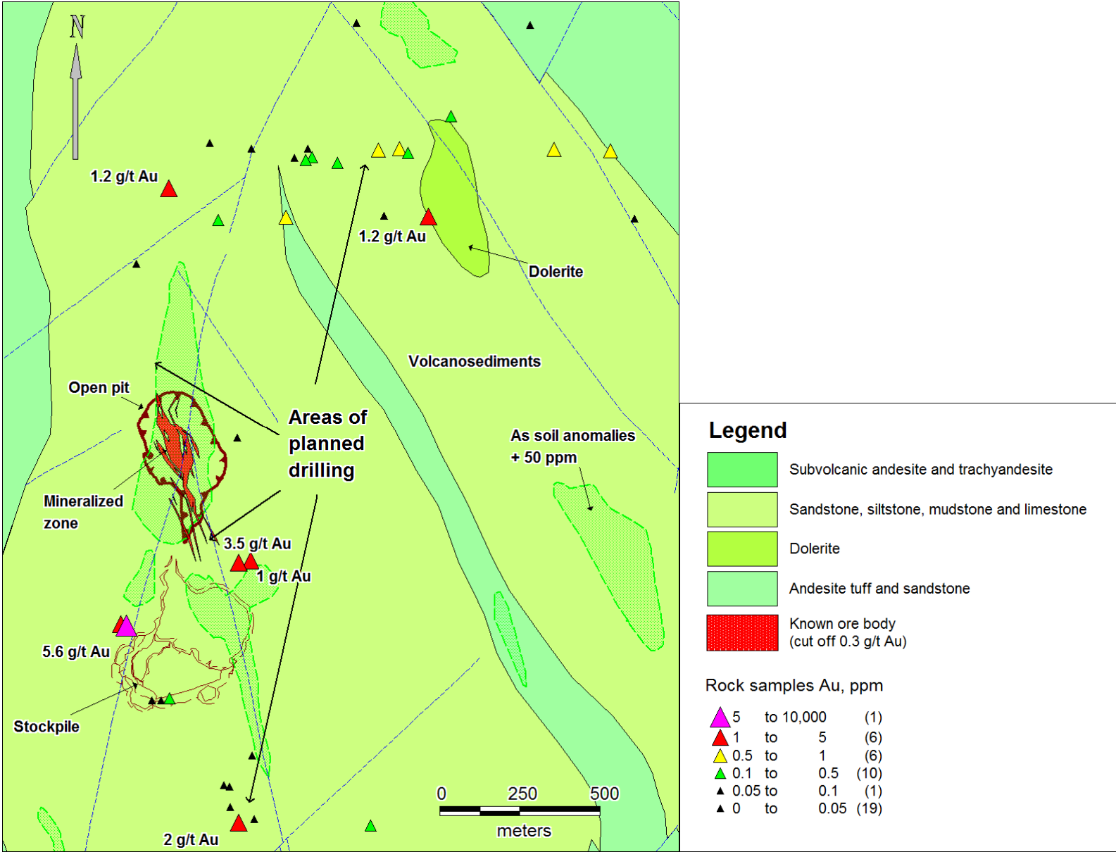
Figure 2 – Dombraly Geological Map with Soil and Rock Sampling Results and 2010 Drilling Program
