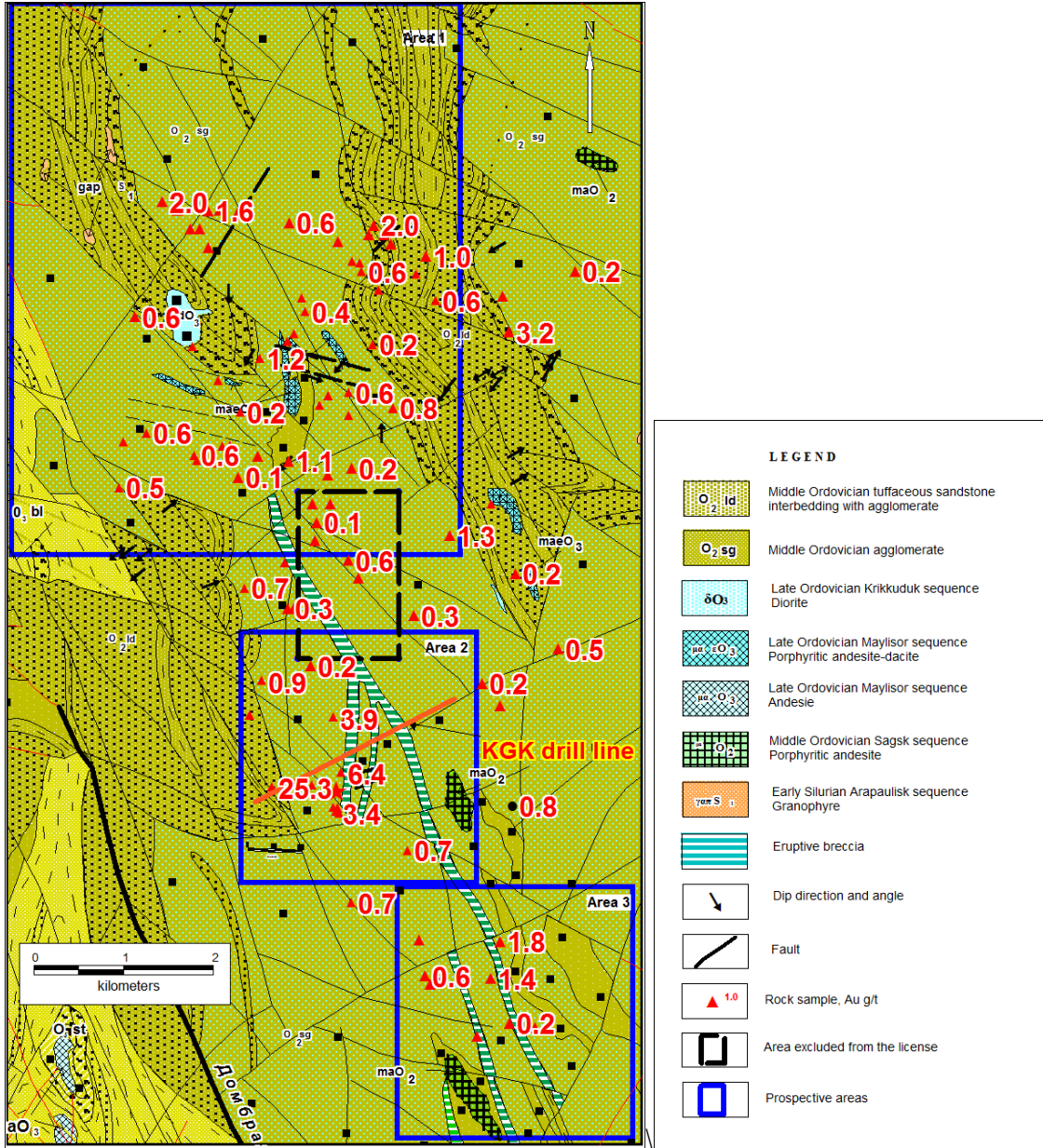
Figure 2 – North Balusty Geological Map with Rock Sampling Results and 2010 Drilling Program
