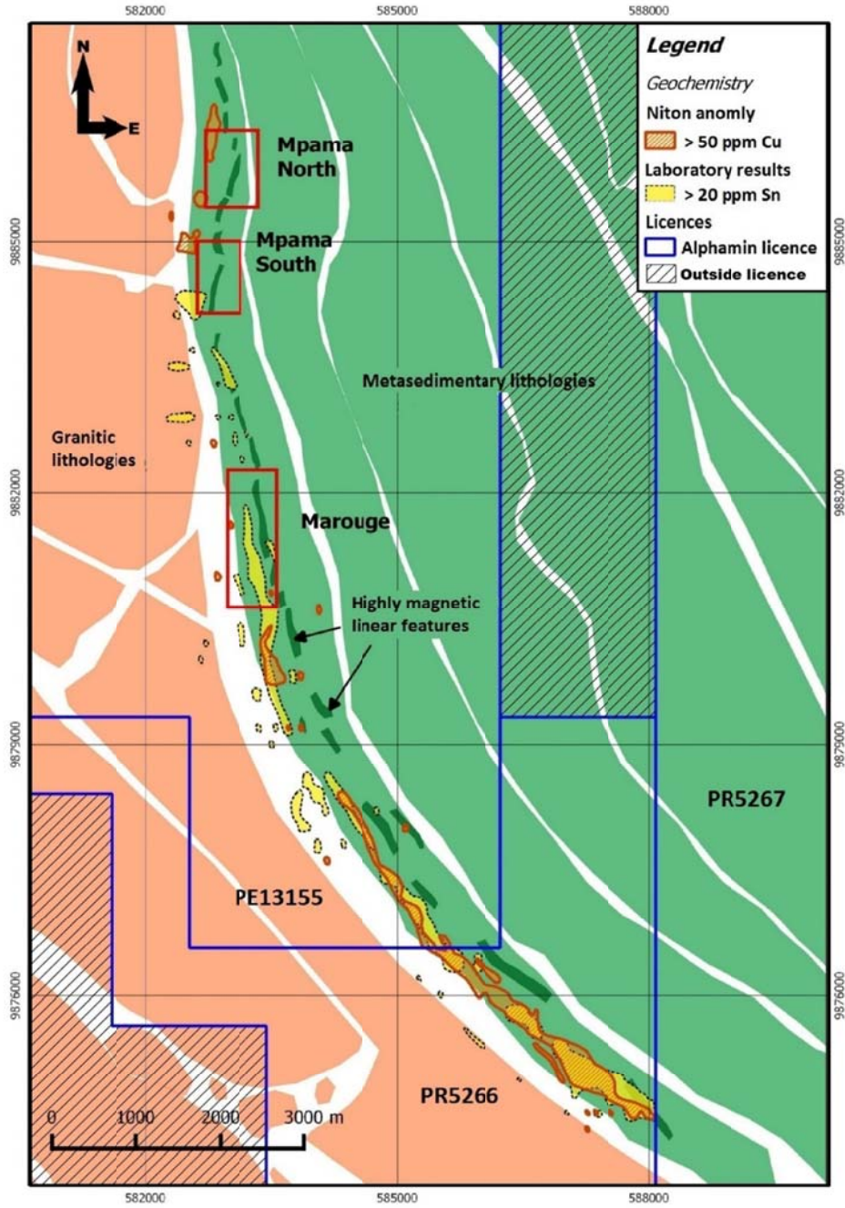
Figure 3: Copper and tin in soil anomalies over Bisie ridge on interpreted geology
