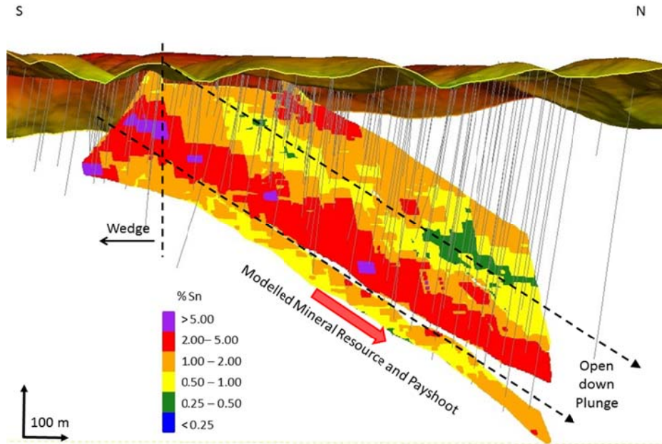
Figure 2: Long Section across Mpama North Orebody showing continuation of high grade mineralisation down plunge.
