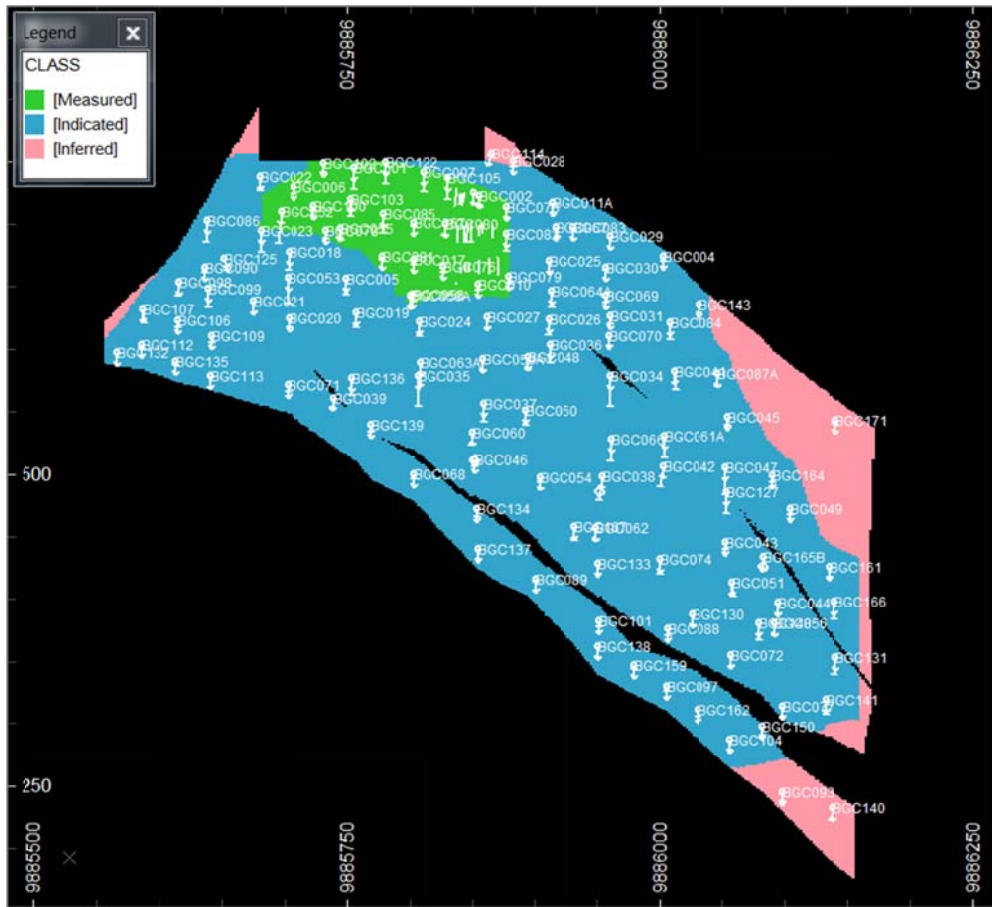
Figure 1: Main Vein Mineral Resource area with Measured, Indicated and Inferred categories shown in green, blue and pink respectively
