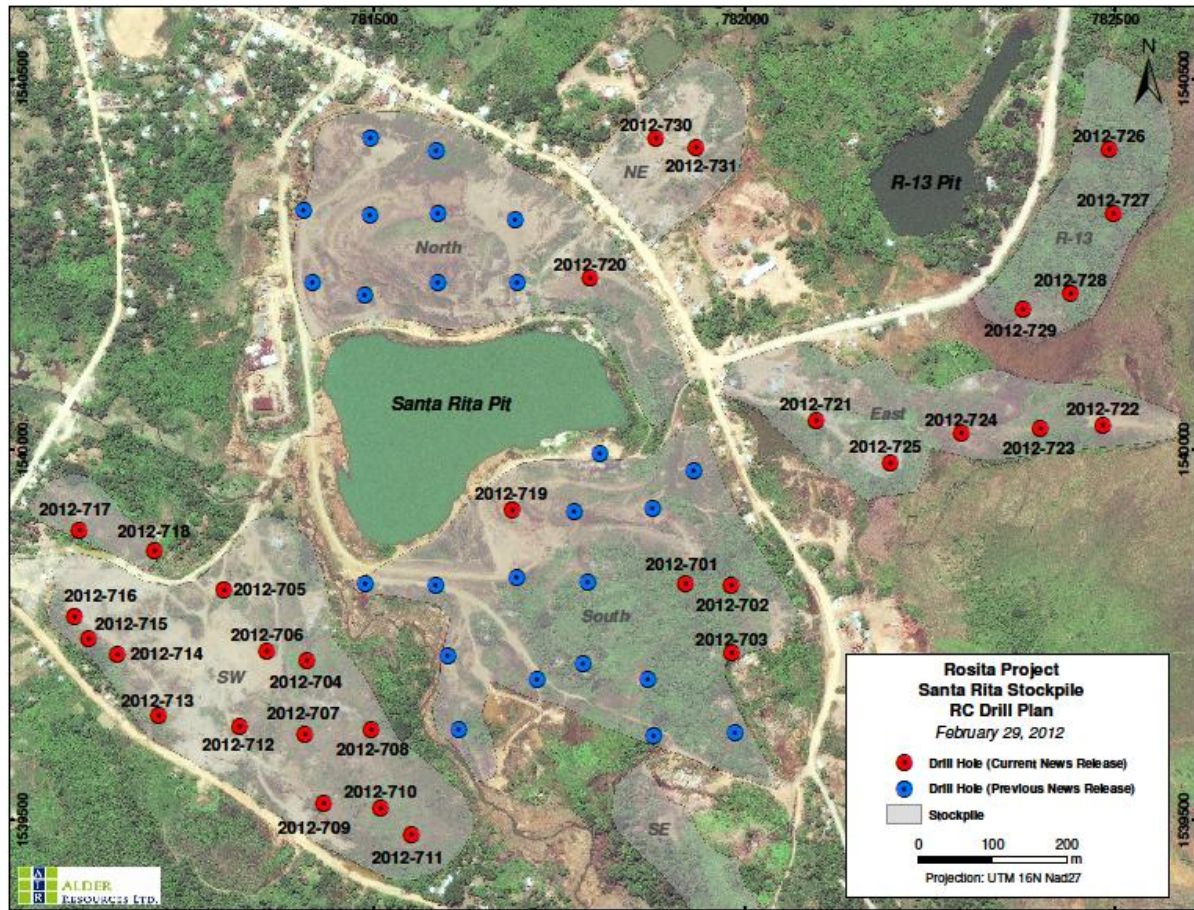
Figure 1. Drill Plan of RC holes at Santa Rita and R-13 areas.
