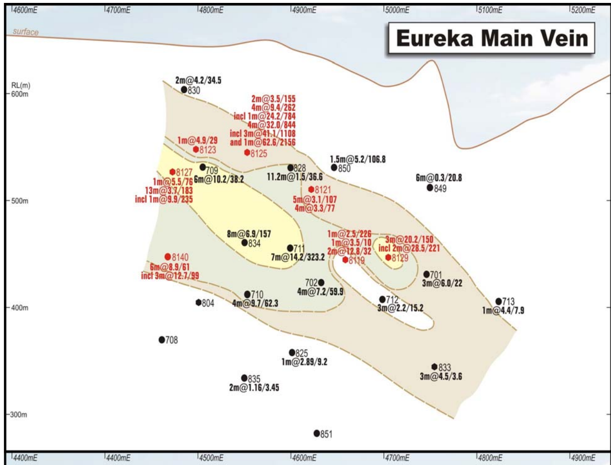
Figure 4: Longitudinal projection of the Eureka Main Vein (Lens 1 – some of the high-grade intercepts correspond to additional lenses within the vein)
