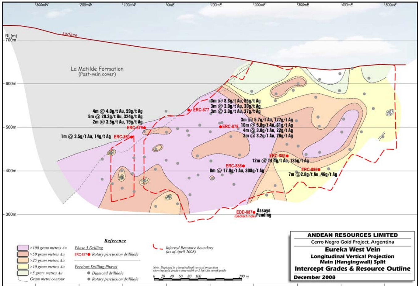
Figure 1: Eureka West Long Section
