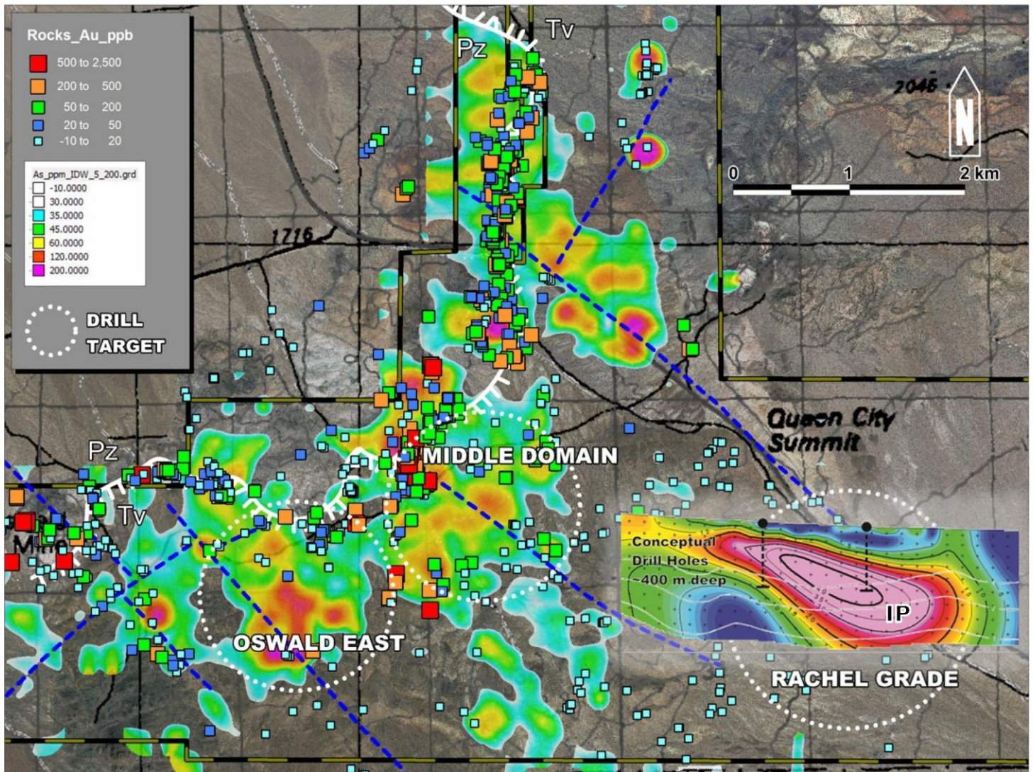
Figure 1. Soil and rock geochemical anomalies showing current drill targets. IP chargeability section inset at Rachel Grade target to scale, showing planned drill holes.
