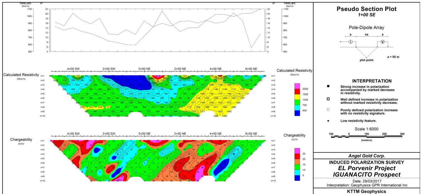
Figure 2: Iguanacito Induced Polarization section 100SE showing on the right of the section an area of strong chargeability (lower pseudosection) at shallow depth flanked to the right by a resistivity anomaly (upper pseudosection).
