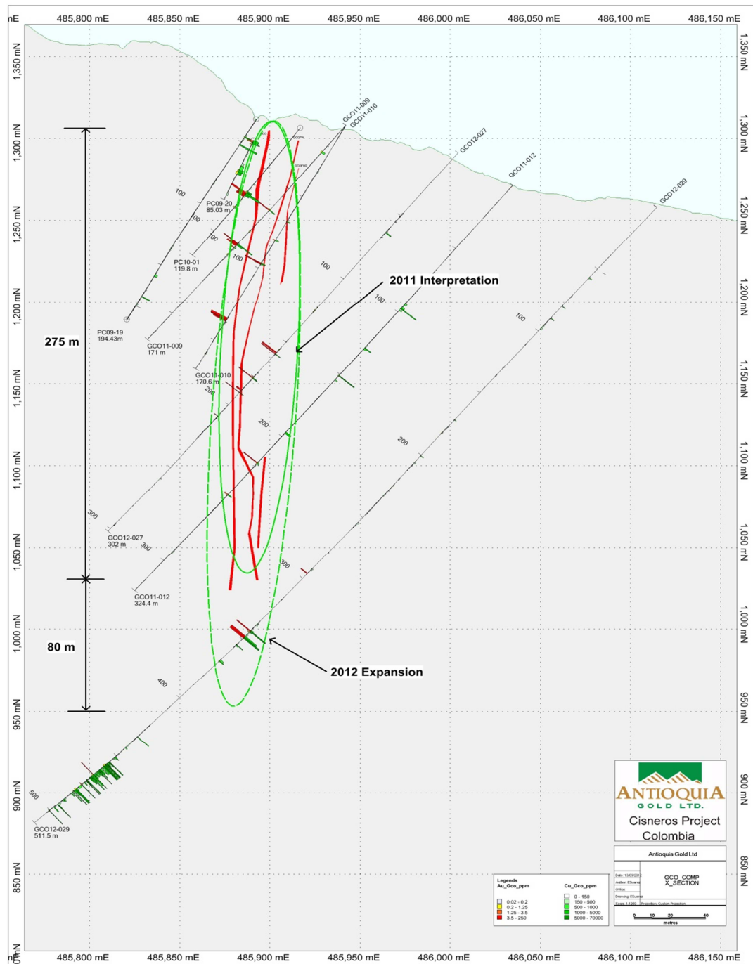
Figure 2 – Guaico Composite Section with the year 2011 and 2012 Depth Interpretation.
