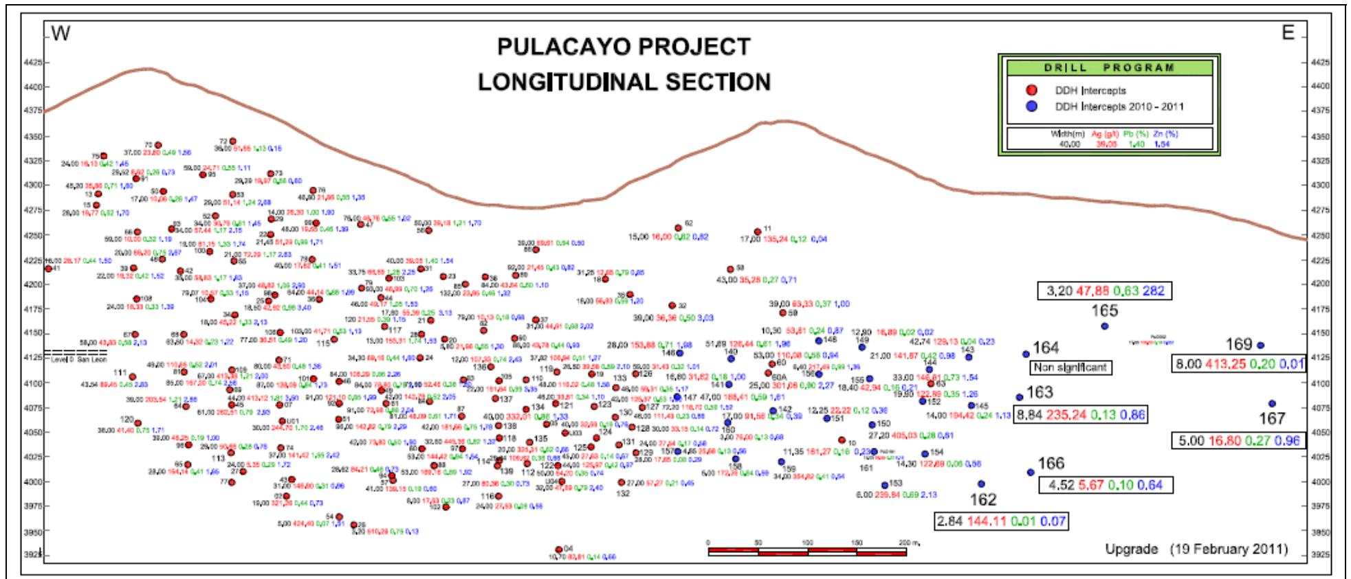
Figure 3 Vertical Longitudinal Section Pulacayo Deposit
