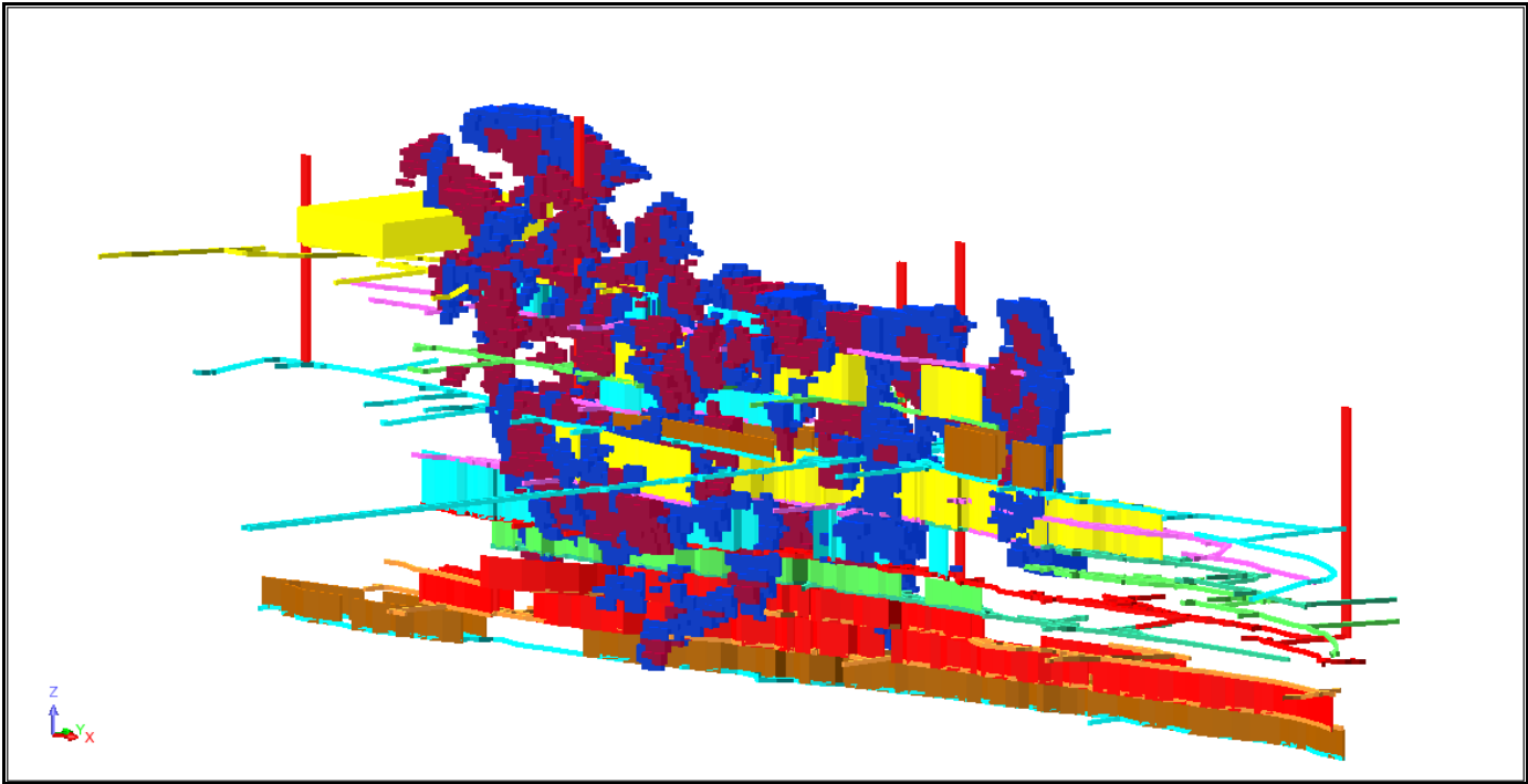
Figure 3b View of Potential Underground Mineral Resources, Looking Northwest, Pulacayo Project. Red=Indicated, Blue=Inferred. Note existing underground workings.(Source: Draft Micon Technical Report, in prep.)
